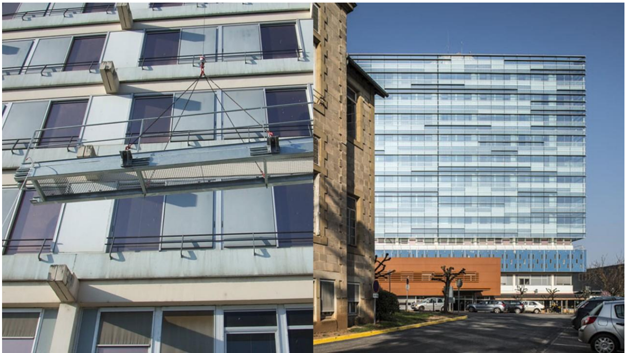
Fig. 1 Brive-la-Gaillarde Hospital, built in 1977 (left picture), and renovated by Vincent Espagno (Espagno Milani Architects) in 2014 (right picture), using a ventilated double-skin facade. Credits: Espagno Milani / Sylvain Mille
